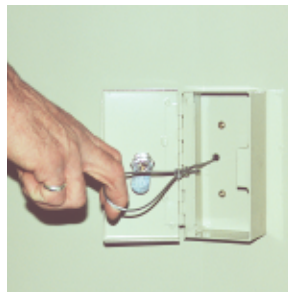
Remote emergency manual lowering device
