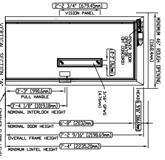
VERTICAL SECTION 'A-A' FLUSH PRO-AUTO DOOR
